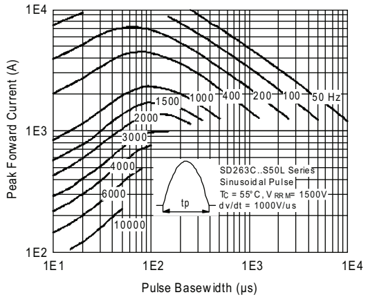
Fig. 16 - Frequency Characteristics
